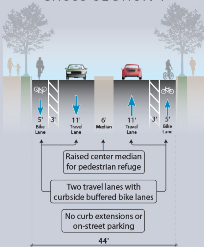
CROSS-SECTION 1
