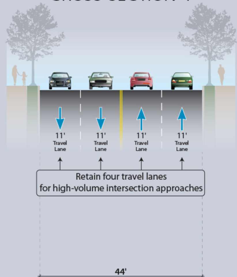
CROSS-SECTION 4
