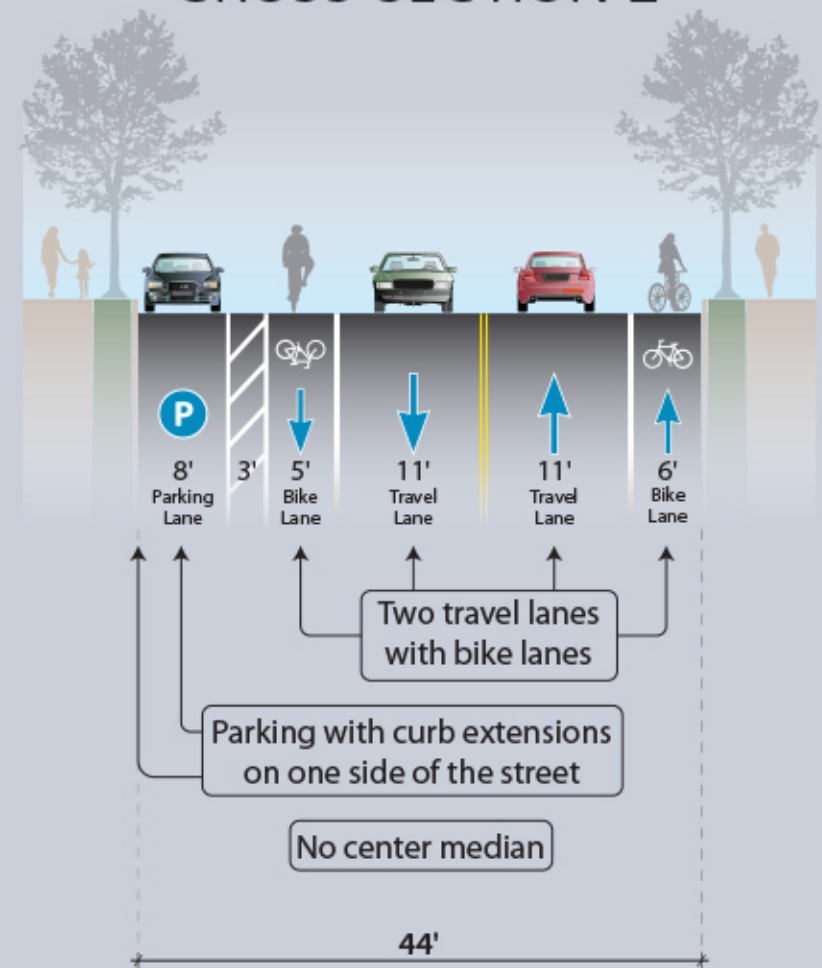
CROSS-SECTION 2
