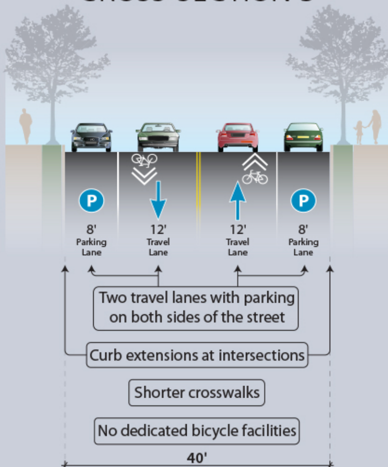
CROSS-SECTION 3
