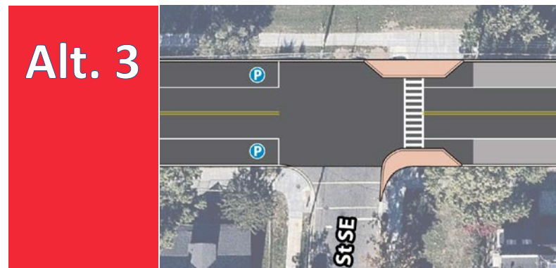
On street parking with neckdowns
