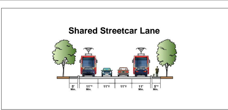
Section FF
